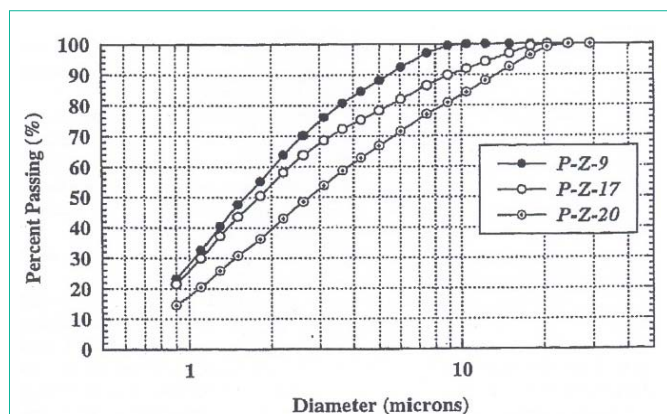
Figure 2: Grain size distribution of the three fine-grained cements [22].
