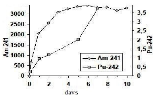
Figure 1: ^{241}\text{Am} и ^{242}\text{Pu} accumulations in Elodea Canadensis biomass.
