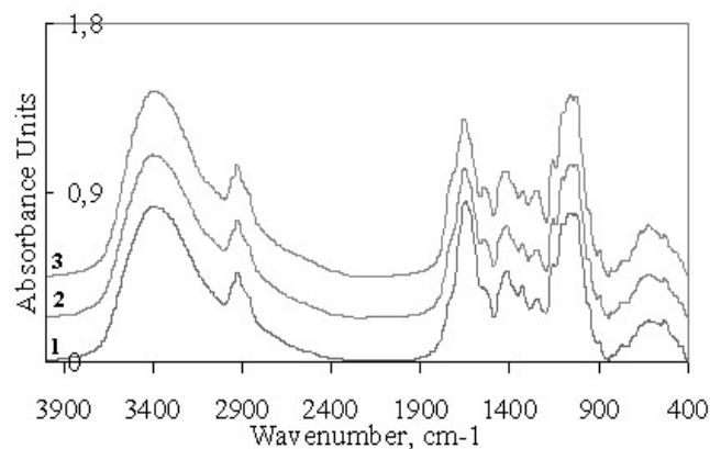
Figure 4: IR spectra of the cellulose samples: curve 1 – control; curve 2 - sample from the system with ^{242}\text{Pu} ( 4\text{ Bq}\cdot\text{sample}^{-1} ); curve 3 - sample from the system with ^{242}\text{Pu} ( 10\text{ Bq}\cdot\text{sample}^{-1} ).
