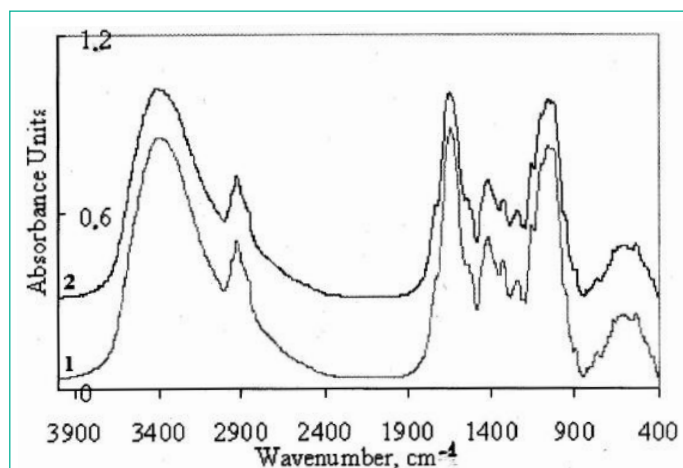
Figure 3: IR spectra of the Elodea samples: 1) control sample; 2) experimental sample.
