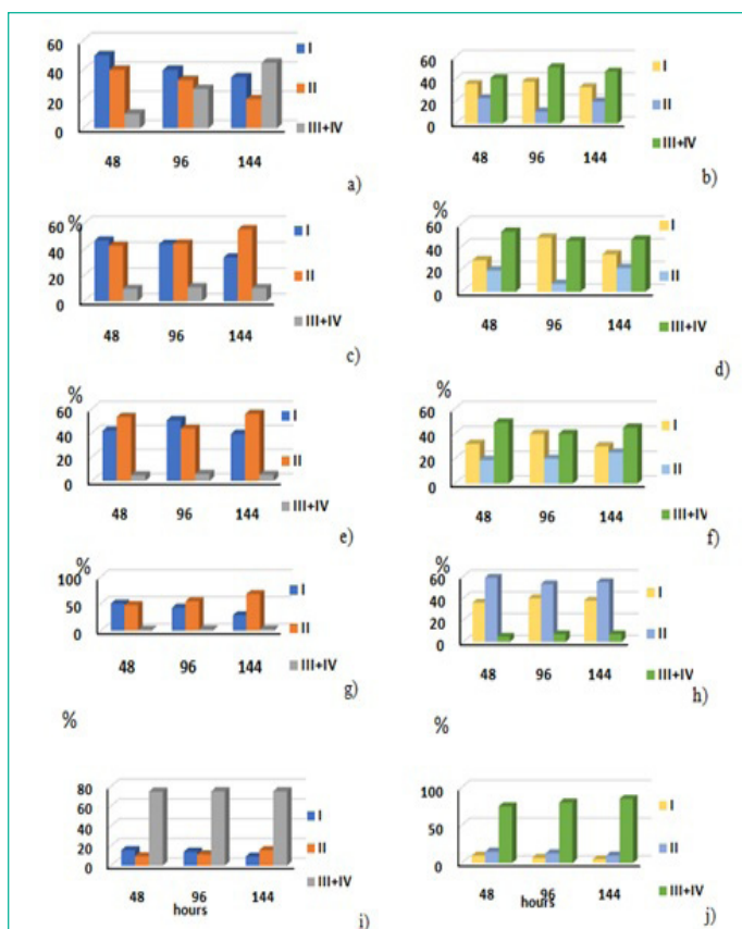
Figure 2: Dynamics of the distribution among the chemical fractions for ^{242}\text{Pu} and ^{241}\text{Am} accumulated by the Elodea biomass in the course of the experiment: I—exchange fraction; II—absorption fraction; III+IV—organic fraction + mineral residue upon the addition of salts of oxalic (c, d), ascorbic (e, f), hydrosulphuric (g, h) and humic acids (i, j) into the systems.
