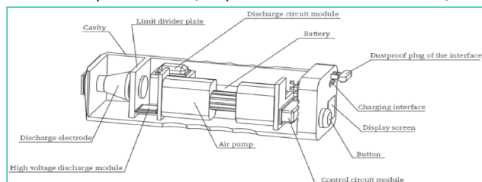
Figure 3: Schematic diagram of the structure of a portable low-temperature air plasma jet coagulation device.
