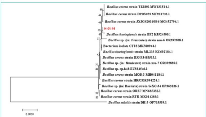
Figure 2: Constructing a phylogenetic tree based on 16S r DNA sequences.
