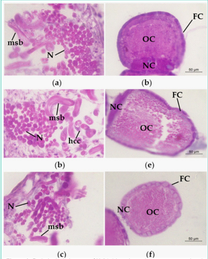
Figure 6: Pathological changes of H-01-14 strain on the spermatozonal and ovarian tissues of S. litura . (a) nest of CK; (b) fine nest of F 0 generation; (c) nest of F 1 generation. (d) ovaries of CK; (e) ovaries of F 0 generation. (f) ovaries of F 1 generation. MSB: mature sperm bundle; N: nucleus; hcc: apical sac cell; OC: oocyte; NC: trophoblast; FC: follicular cells.
