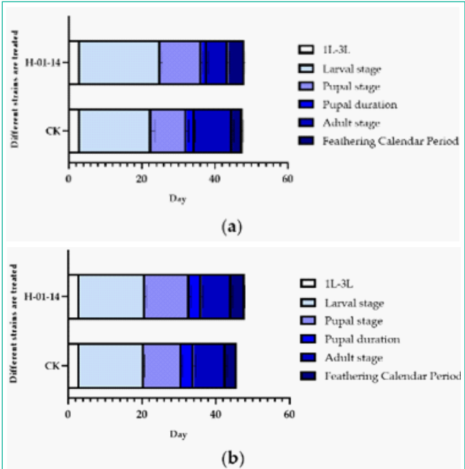
Figure 3: (a) Effects of different strains on the development duration of F 0 ; (b) Effects of different strains on the development duration of S. litura .
