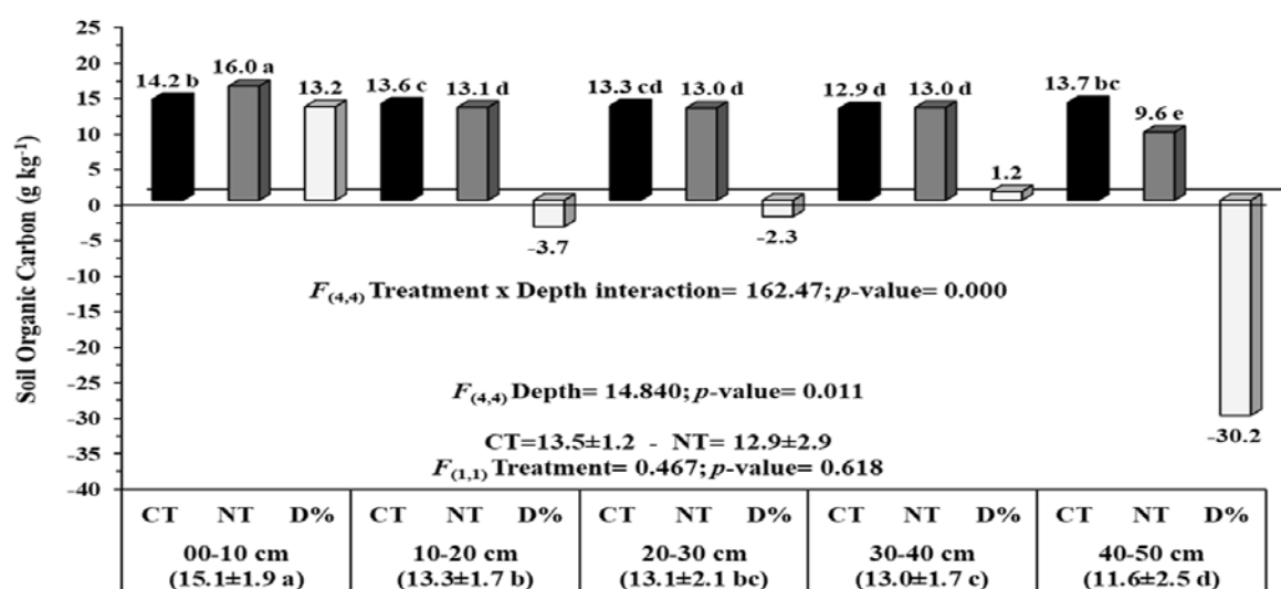
Figure 4: Soil organic carbon values for No-Tillage (NT, gray bars) and Conventional Tillage (CT, black bars) measured in October at five depths (10-20-30-40-50 cm) during the 2008 and 2009 growing seasons. For NT and CT treatments and soil depth levels, the values are the mean ( n=20 and n=8 , respectively) \pm standard deviation. Different lowercase letters next to the means indicate a significant difference at P=5\% , according to the Least Significant Different test. For the treatment x depth interaction, D% (white bars) represents the difference, expressed as a percentage, between the NT and CT treatments.
