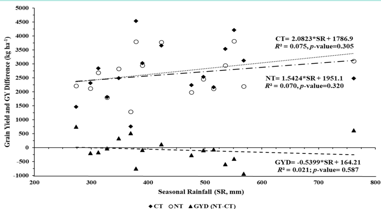
Figure 2: Linear regression performed between the grain yields (GY) of No-Tillage (NT), Conventional Tillage (CT) and difference (GYD) between NT and CT treatments and total Seasonal Rainfall (mm) recorded from October to June of each year.
