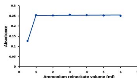
Figure 4: Stoichiometry of the reaction of lomefloxacin hydrochloride (2.6 x 10 -2 M) with ammonium reineckate (2.6 x 10 -2 M) by molar ratio method.
