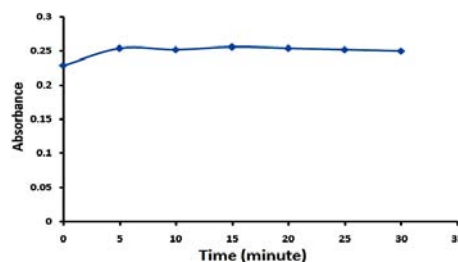
Figure 3: Effect of time required for complete reaction of lomefloxacin (100µg/ml) and ammonium reineckate (10 -2 M).
