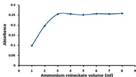
Figure 2: Effect of volume of ammonium reineckate (10 -2 M) on the absorbance of its reaction product with lomefloxacin hydrochloride (100µg/ml).
