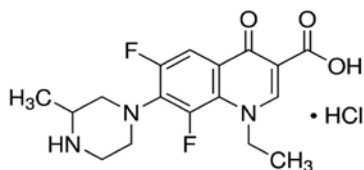
Figure 1: Structural formula of lomefloxacin hydrochloride.
