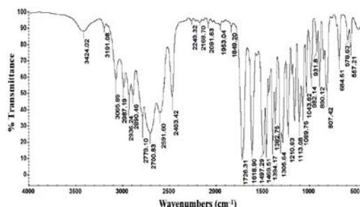
Figure 5: IR spectrum of lomefloxacin hydrochloride.
