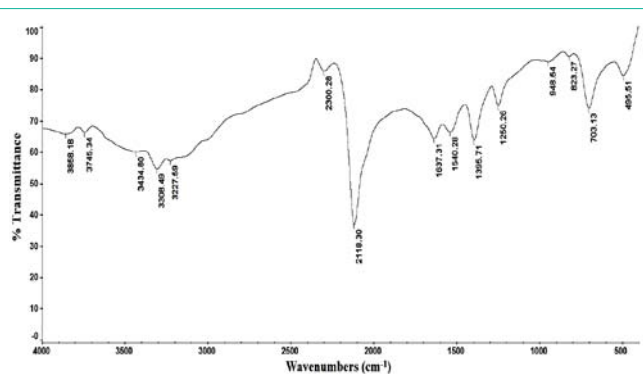
Figure 6: IR spectrum of ammonium reineckate.
