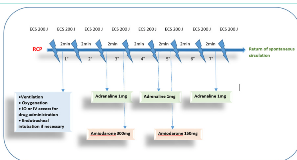
Figure 3: Shockable rhythm management algorithm based on the SFAR [14].
