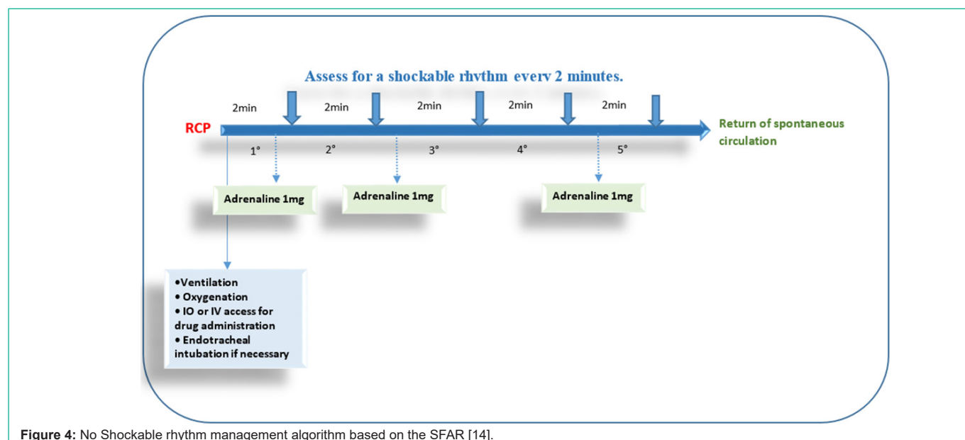
Figure 4: No Shockable rhythm management algorithm based on the SFAR [14].
