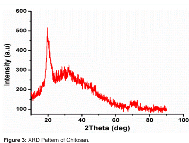
Figure 3: XRD Pattern of Chitosan.
