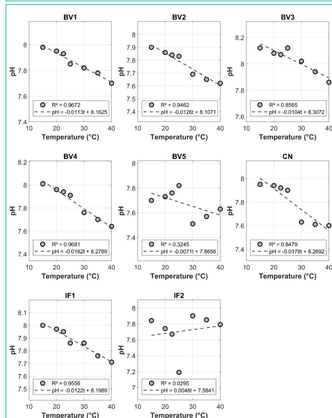
Figure 2: Relationship between temperature ( ^{\circ}\text{C} ) and pH (mol/kg-sol) at sampling sites BV1, BV2, BV4, IF1, BV3, BV5, CN, and IF2 (linear regression, significance level p < 0.05 ). Each panel reports the significant linear equation and the coefficient of determination ( R^2 ).
