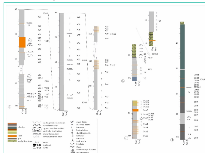
Figure 6: Lithostratigraphic columns of the studied surface appearance (a) along the Xi beach; (b) Koutala beach; (c) Matzavinata; (d) Chavdata. The numbers of the analyzed samples are also noted next to the columns.
