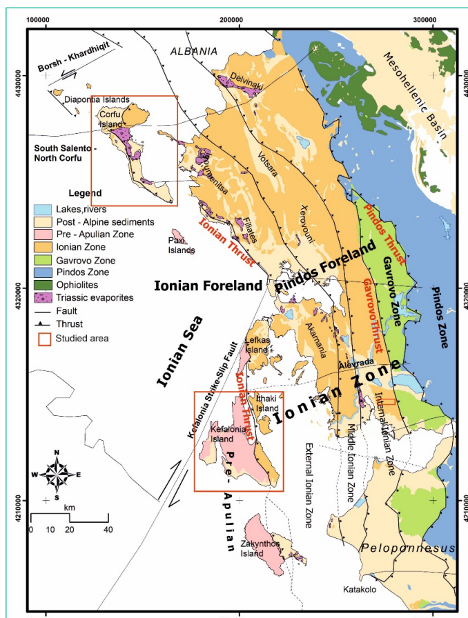
Figure 1: Geological map of Western Greece where the two research areas (Kefalonia and Corfu Islands) are marked with a red box [18,19].
