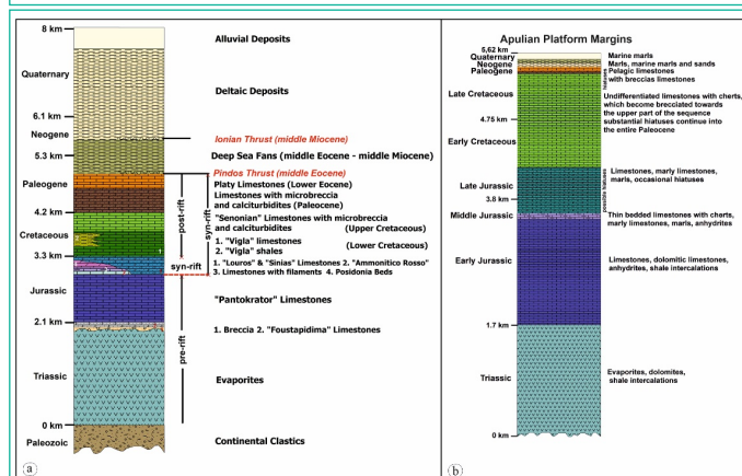
Figure 2: The stratigraphic columns of the (a) Ionian basin; (b) Apulian platform margins [18,19].
