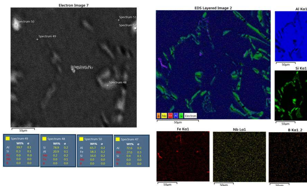
Figure 3: SEM-EDS of various spots on the Al10Si1Fe alloy sample with the addition of the inoculant Nb+B.
