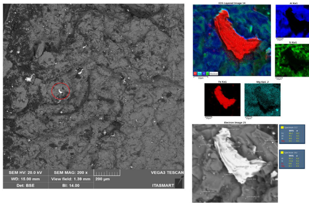
Figure 9: SEM-EDS showing the morphology of the deformed \beta -Fe precipitates after solubilization and precipitation treatment, found on the surface of the fractured CDP face.
