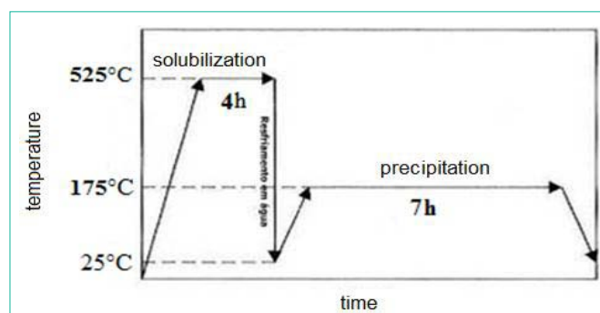
Figure 1: Solubilization treatment followed by rapid cooling and precipitation.
