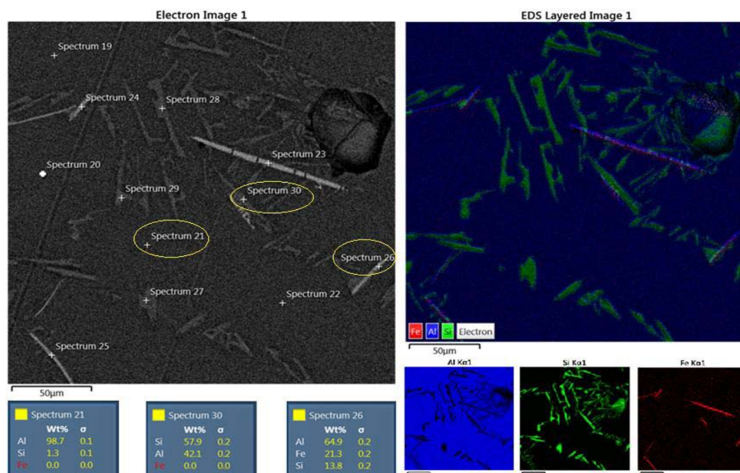
Figure 2: SEM-EDS of various spots on the Al10Si1Fe alloy sample.
