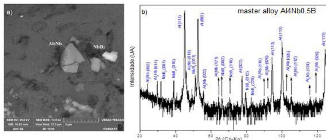
Figure 4: a) \text{Al}_3\text{Nb} and \text{NbB}_2 substrates found by SEM-EDS, identified by image similarity, and b) Characterization of the substrates by XRD on the \text{Al4Nb0.5B} master alloy.
