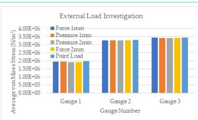
Figure 10: External load investigation.
