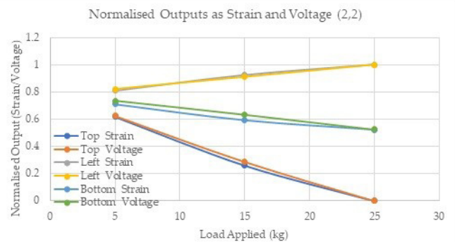
Figure 22: Comparison of sensor outputs as strain (strain indicator) and voltage (self-made PCB) from point (2,2).
