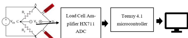
Figure 18: Electronics configuration.
