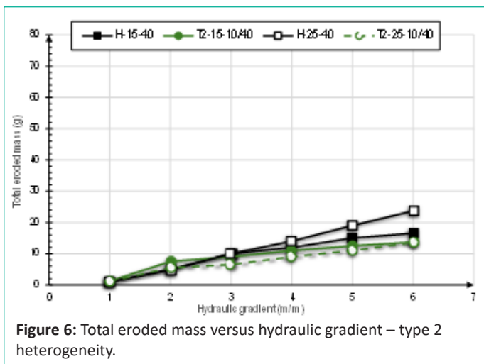
Figure 6: Total eroded mass versus hydraulic gradient – type 2 heterogeneity. However, a reduction in the eroded mass is observed when the density index increases from 0.1 to 0.4; this decrease is more than 39% for heterogeneous samples (containing 25% of erodible fines) and approximately 21% for homogeneous ones (with 25% erodible fines). This drop in eroded mass with the increase in the density index could be due to the reduction in pore space locally inducing clogging phenomena.
