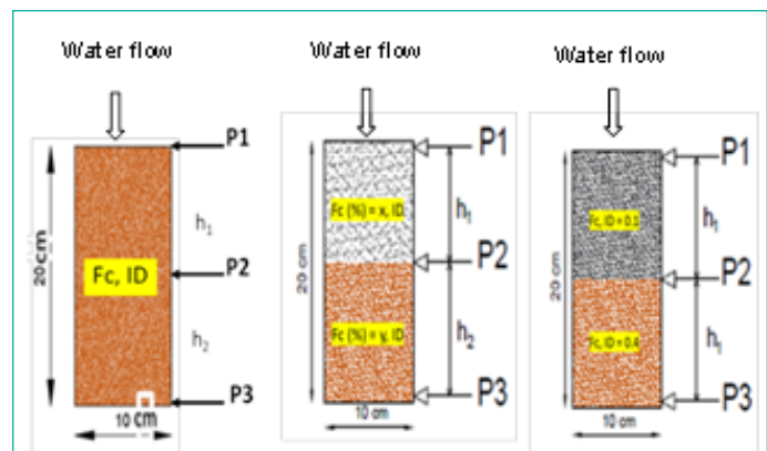
Figure 3: Configuration of studied specimens. (a) Homogeneous sample considered as control specimen; (b) Fine particle content heterogeneity ( F_c ); (c) Compaction heterogeneity ( I_D ).
