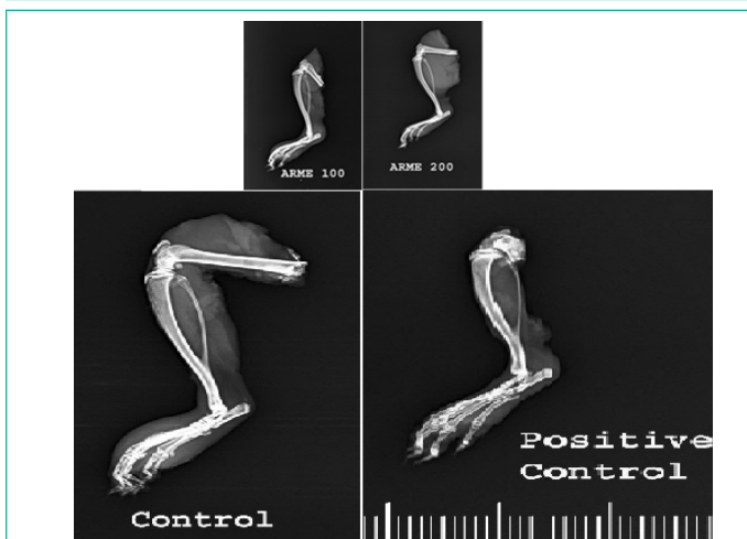
Figure 5: FCA induced Arthritis – Radiography.
