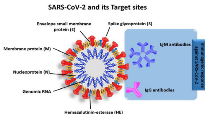
Figure 1: SARS-CoV-2 schematic structure and possible diagnostic targets: Reprint and permission from ref [31]. Copyright 2020 King Abdulaziz City for Science and Technology.
