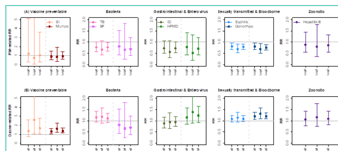
Figure 1: Relative risk (and 95% CIs) of air pollutant related infectious disease per 10 \mu\text{g}/\text{m}^3 increase in \text{PM}_{2.5} and \text{O}_3 for each category of NNIDs. The double-pollutant DLM model was adjusted for seasonality and long-term trend, other air pollutant, mean temperature, and relative humidity.
